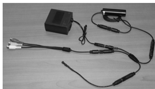
Figure 12 Complete DT-CAME580 Modular Ultra Hi-Res Helmet Camera Kit w/ RCA recording cable and Covered 8-AA Battery Pack
