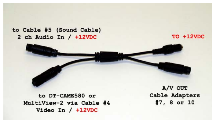
Figure 5 Modular A/V Harness
